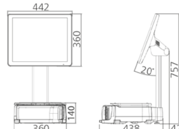
SM-5300SSP (19" Self-Service)
