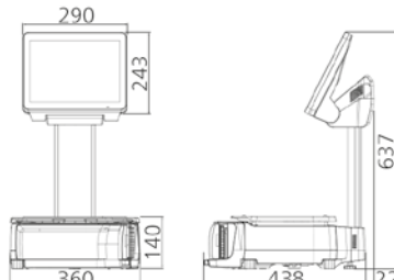
SM-5300SSP (12.1" Self-Service)
