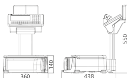
SM-5300EV (Elevated)
