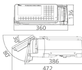
SM-5300EV (Elevated)
