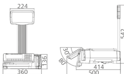
SM-5300SSP (12.1" Self-Service)
