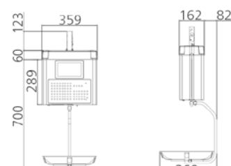
SM-5300SSP (19" Self-Service)
